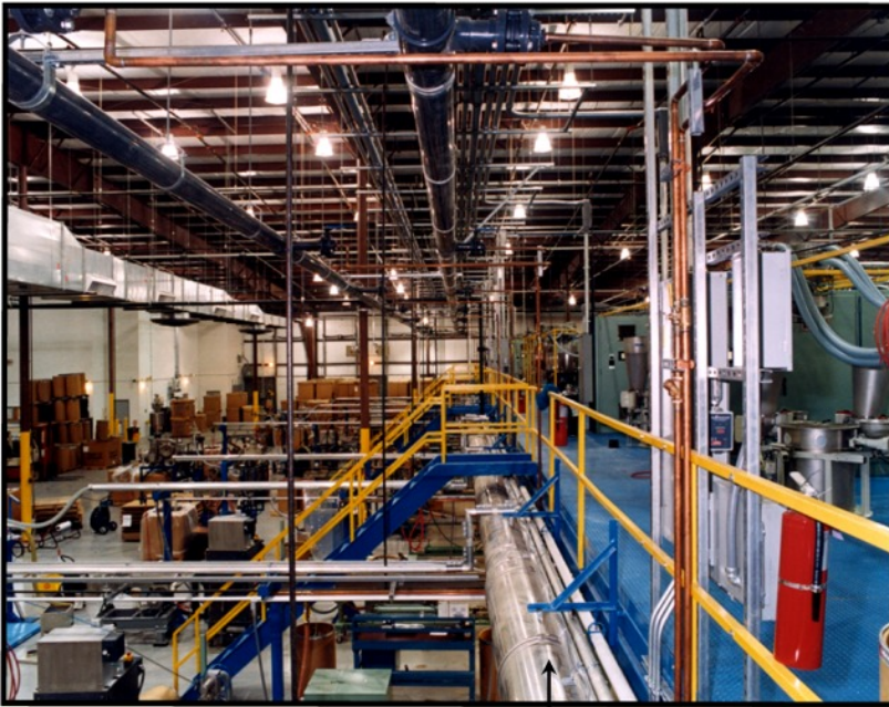
Fume Exhaust System with Scubbers
